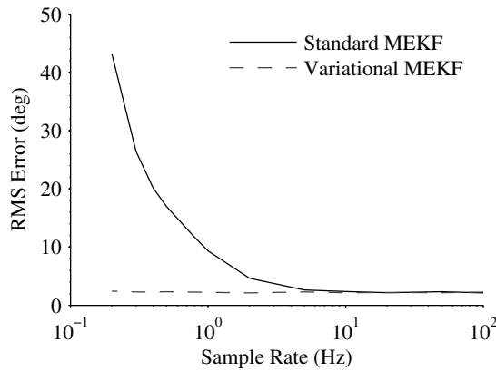
Figure 7. Multiplicative extended Kalman filter RMS attitude error
