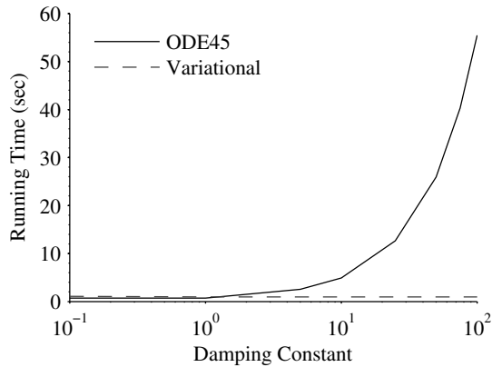
Figure 4. Integrator running time
