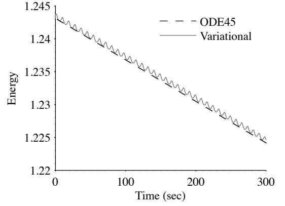
Figure 5. Energy for rigid body with damper
