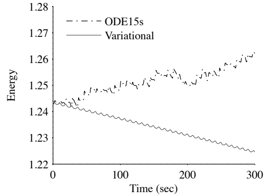
Figure 6. Energy for rigid body with damper
