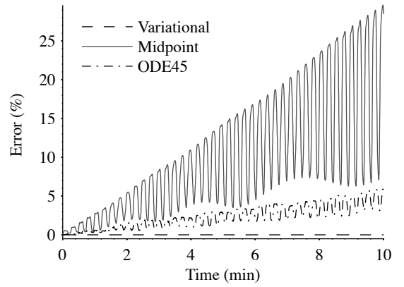
Figure 1. Momentum error for a free rigid body
