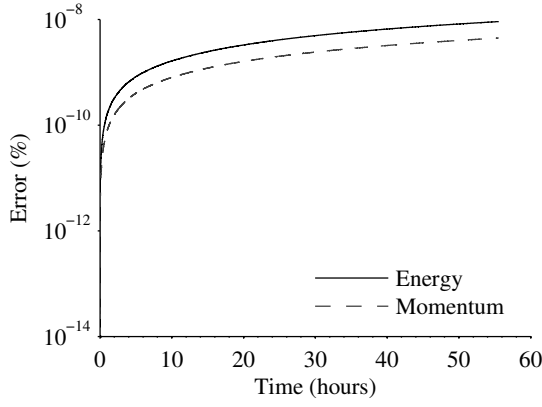
Figure 3. Long-term error for a free rigid body
