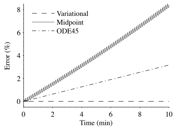
Figure 2. Energy error for a free rigid body
